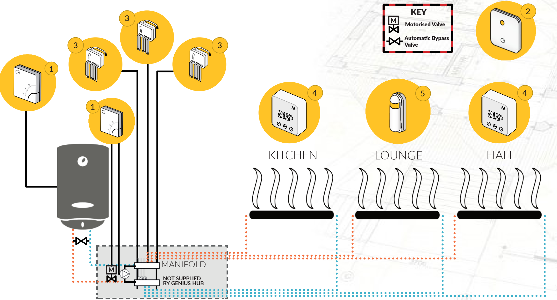
1 - Electric Switch | 2 - Genius Hub | 3 - Electric Relay | 4 - Room Thermostat | 4 - Room Sensor
